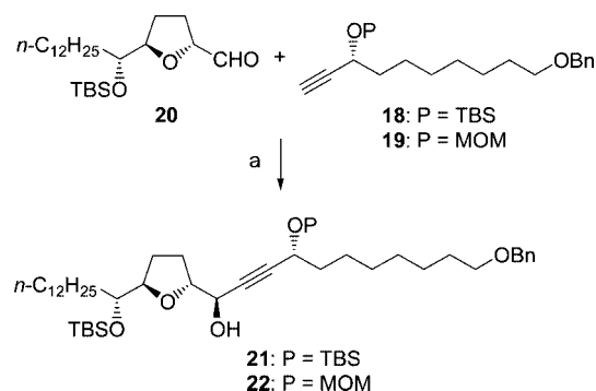
Scheme 6. Asymmetric alkynylation of alkynes 18 and 19 : a) \text{Zn}(\text{OTf})_2 , \text{Et}_3\text{N} , (1 R ,2 S )-(-)- N -methylephedrine, toluene, room temp., 21 (0%), 22 (89%), \beta\text{-OH}/\alpha\text{-OH} > 97:3 .
