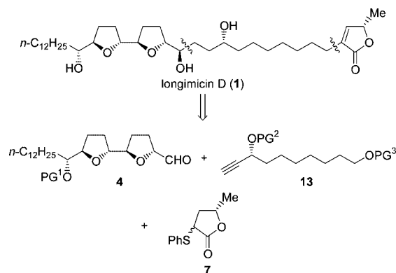
Scheme 4. Alternate retrosynthetic analysis of longimicin D.
