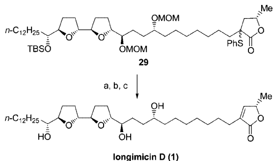
Scheme 9. Synthesis of longimicin D: a) m -CPBA, CH 2 Cl 2 , 0 °C, b) toluene, reflux, c) AcCl, MeOH, CH 2 Cl 2 , room temp., 71% in three steps.
