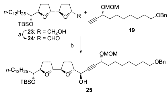
Scheme 7. Asymmetric alkynylation of aldehyde 24 with alkyne 19 : a) \text{SO}_3\cdot\text{pyridine} , DMSO, \text{Et}_3\text{N} , \text{CH}_2\text{Cl}_2 , 0^{\circ}\text{C} to room temp., 90%, b) \text{Zn}(\text{OTf})_2 , \text{Et}_3\text{N} , (1 R ,2 S )-(-)- N -methylephedrine, toluene, room temp., 65%, \beta\text{-OH}/\alpha\text{-OH} > 97:3 .
