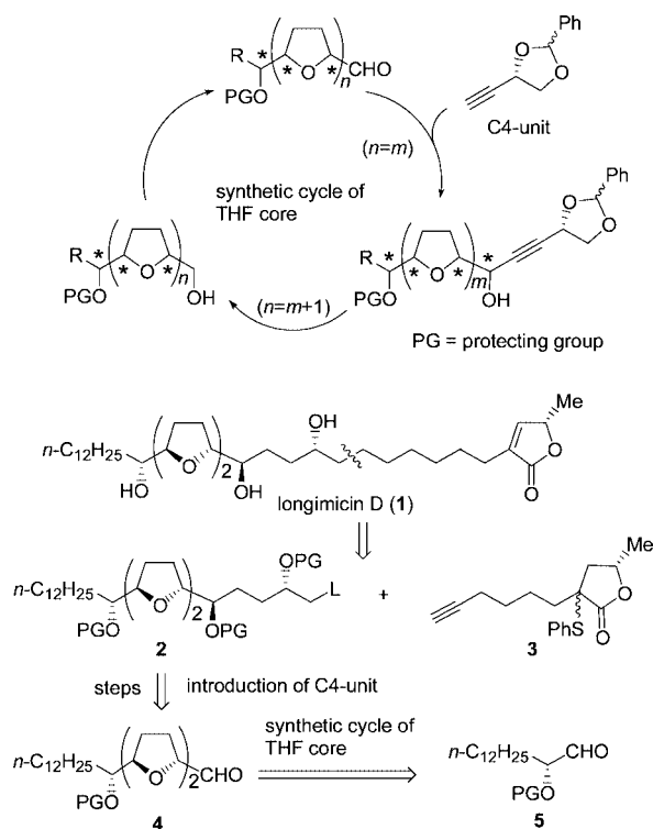
Scheme 2. Synthetic cycle for poly-THF cores and retrosynthetic analysis of longimicin D.
