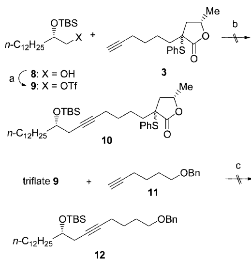
Scheme 3. Alkynylation of 9 with 3 or 11: a) \text{Tf}_2\text{O} , 2,6-lutidine, \text{CH}_2\text{Cl}_2 , 0 °C, quant., b) n\text{-BuLi} , THF, -78 °C, c) n\text{-BuLi} , HMPA, THF, -78 °C to room temp.
