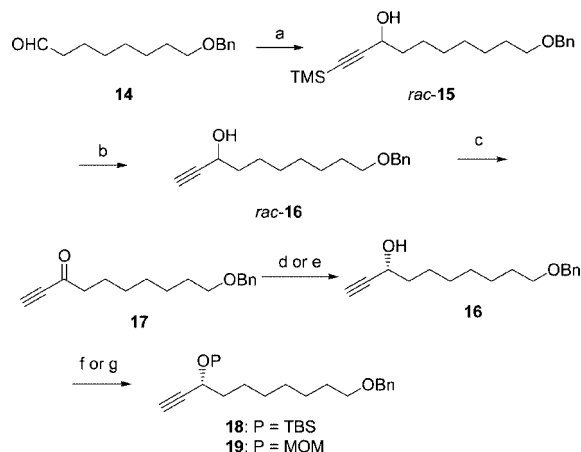
Scheme 7. Asymmetric alkynylation of aldehyde 24 with alkyne 19 : a) \text{SO}_3\cdot\text{pyridine} , DMSO, \text{Et}_3\text{N} , \text{CH}_2\text{Cl}_2 , 0^{\circ}\text{C} to room temp., 90%, b) \text{Zn}(\text{OTf})_2 , \text{Et}_3\text{N} , (1 R ,2 S )-(-)- N -methylephedrine, toluene, room temp., 65%, \beta\text{-OH}/\alpha\text{-OH} > 97:3 .
