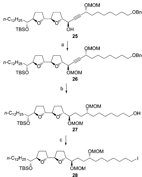
Scheme 8. Preparation of bis-THF ring segment 28 : a) MOMCl, i Pr 2 NEt, \text{CH}_2\text{Cl}_2 , 0^{\circ}\text{C} to room temp., 94%, b) \text{H}_2 , 10% Pd/C, EtOAc, room temp., 73%, c) \text{I}_2 , PPh 3 , imidazole, \text{CH}_2\text{Cl}_2 , 0^{\circ}\text{C} to room temp., 82%.
