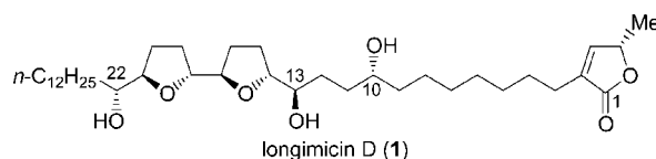
Scheme 1. Structure of longimicin D.
